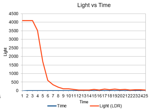
Figure 9: Light Variation across Time
